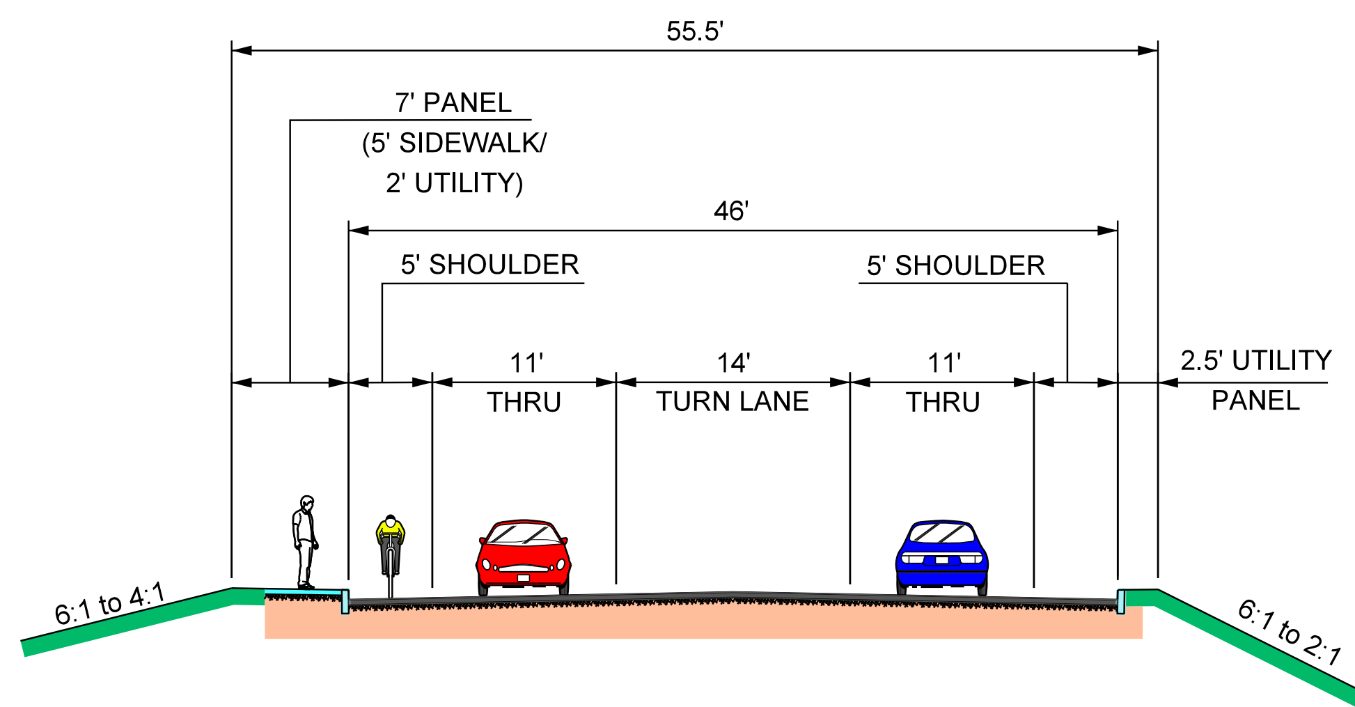
3-LANE TYPICAL TSIENNETO ROAD
