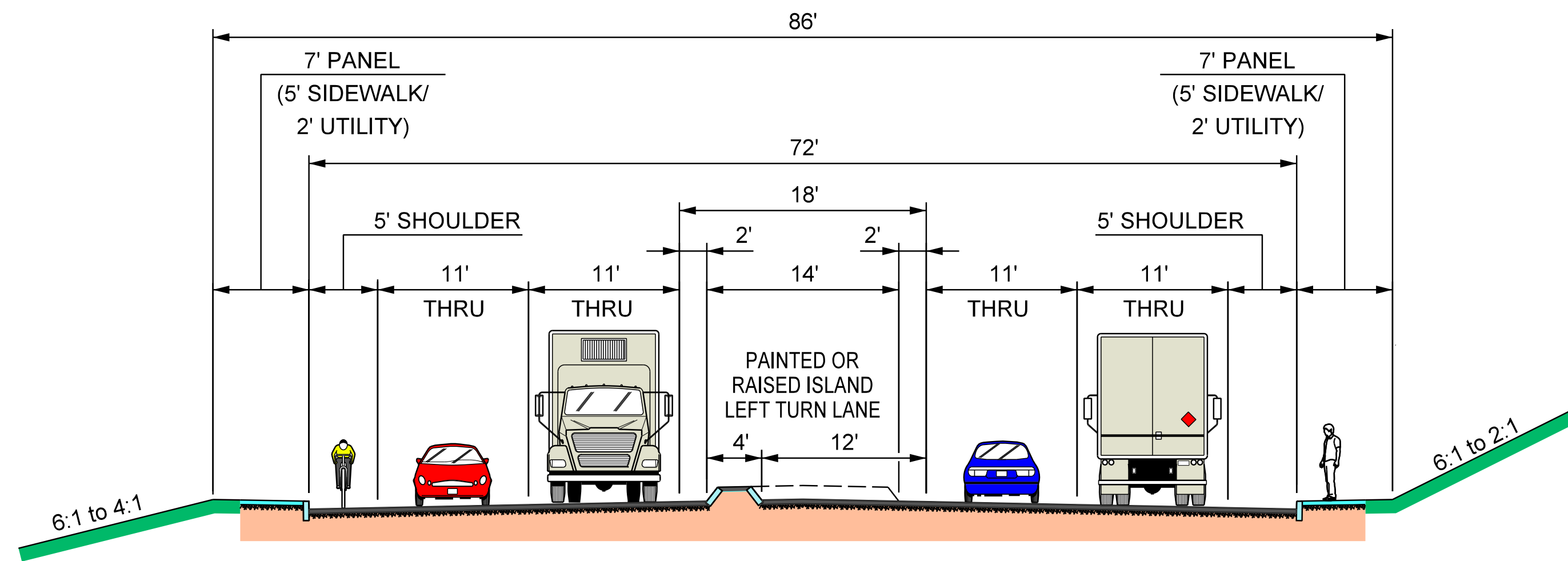
5-LANE TYPICAL CONNECTOR ROAD ROUTE 28 FOLSOM ROAD
